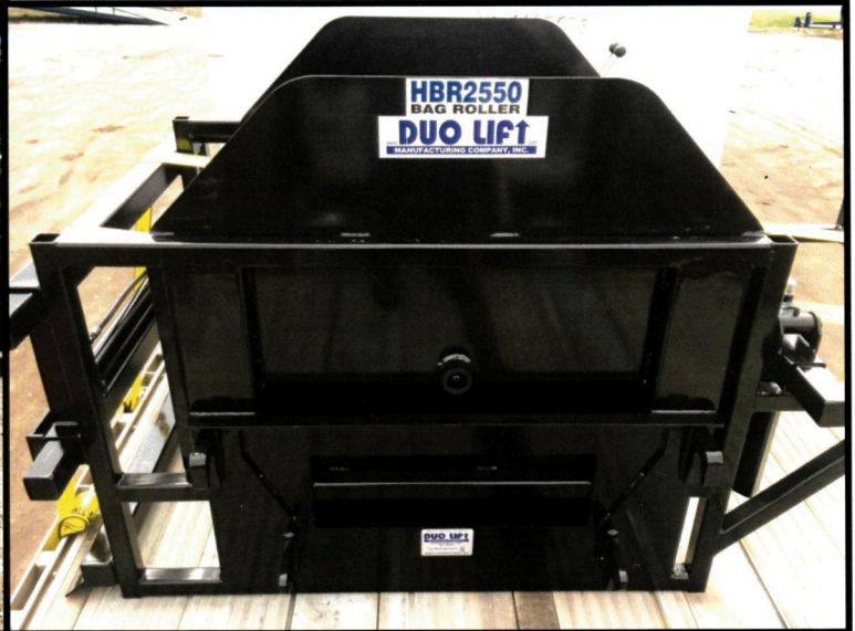
801340 Euro/Global Farm Loader Mounting Plate Welded to RH Side of Main Frame
